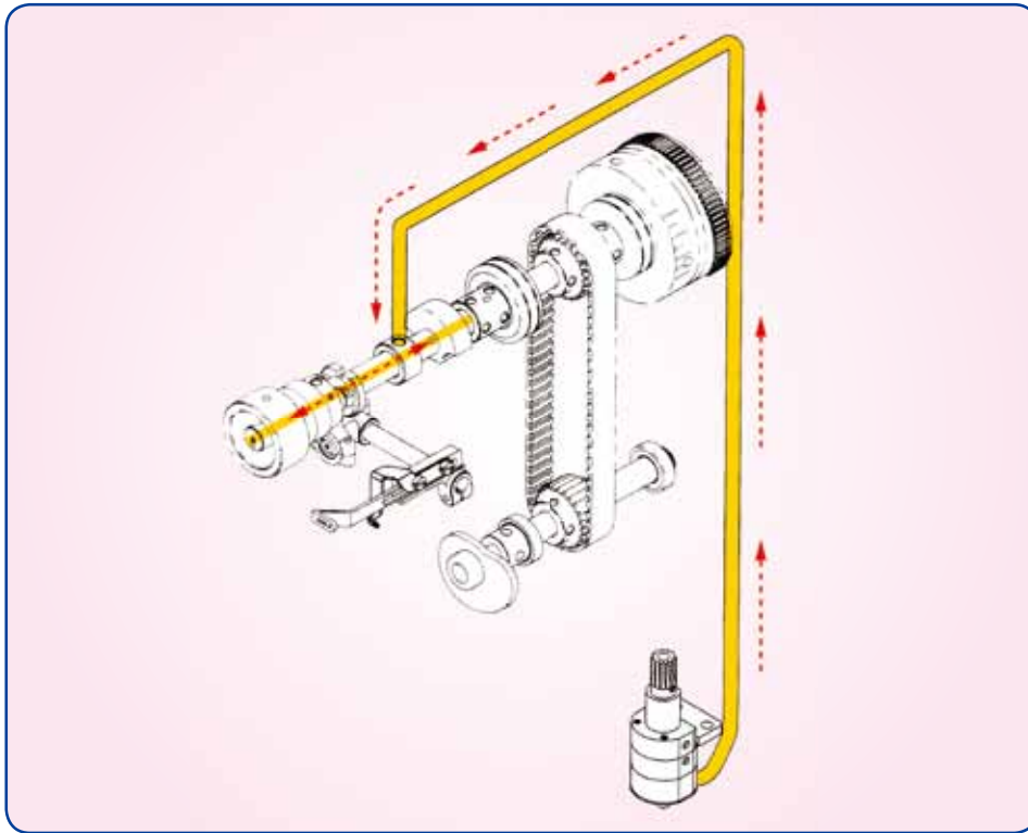
強制給油裝置 Fully-automatic lubrication system
