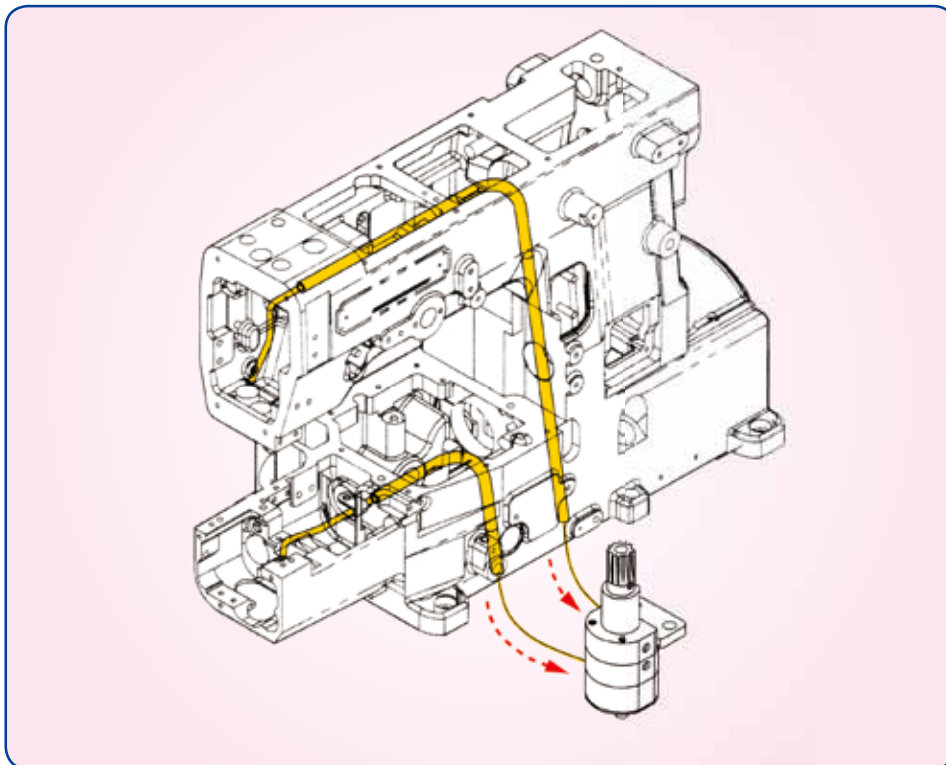
回收油裝置 Recycling lubrication system
